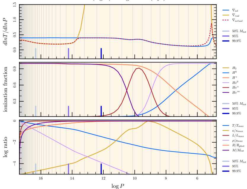
Profiles ( \log P ) — Age 4.556 (Gyr)
