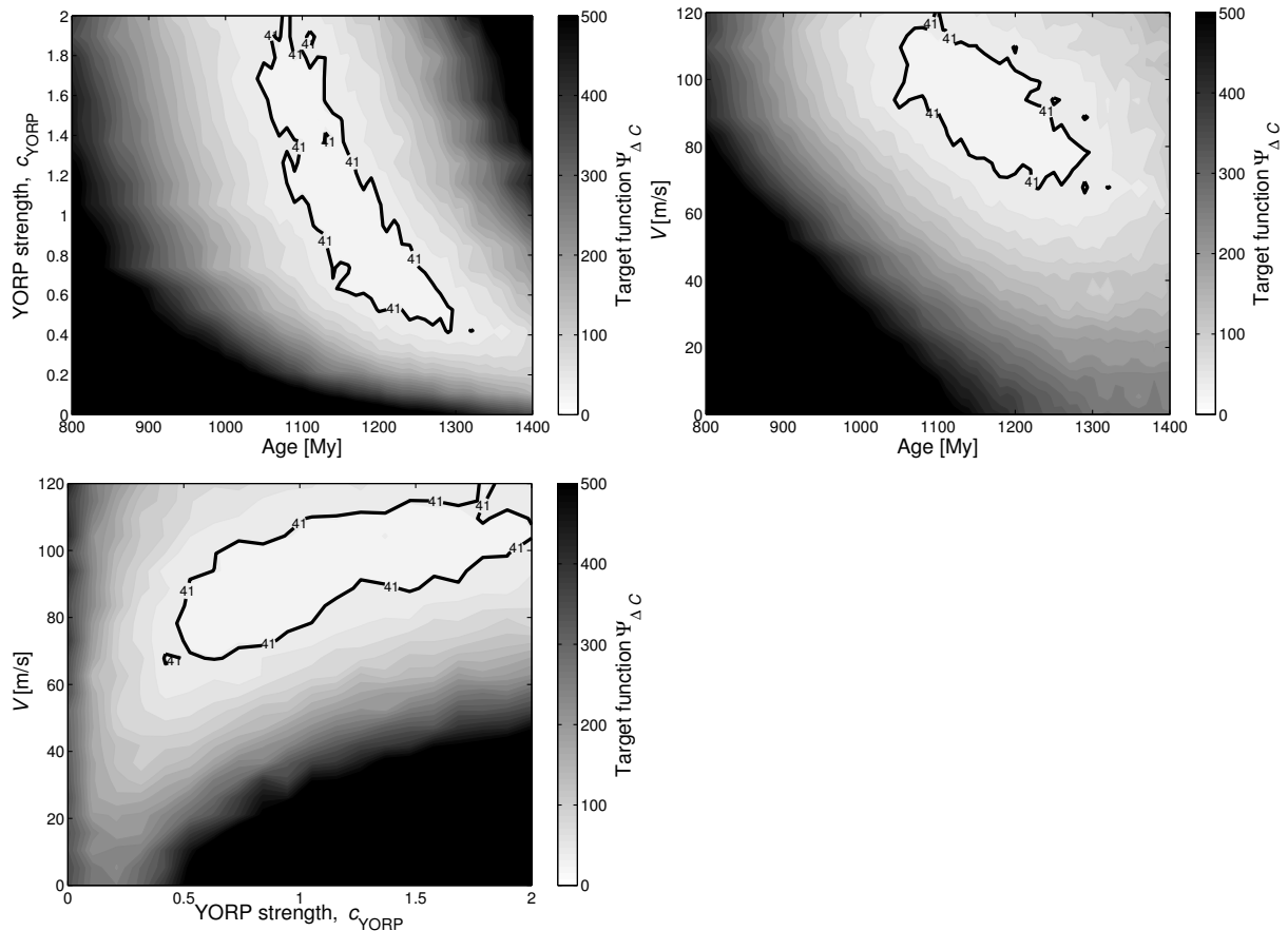
Figure 84: The same as in Fig. 82 but here for the model where V_{SD} = V (5 km/D) is size-dependent. The best-fit value is \Psi_{\Delta C} = 26.2 .
