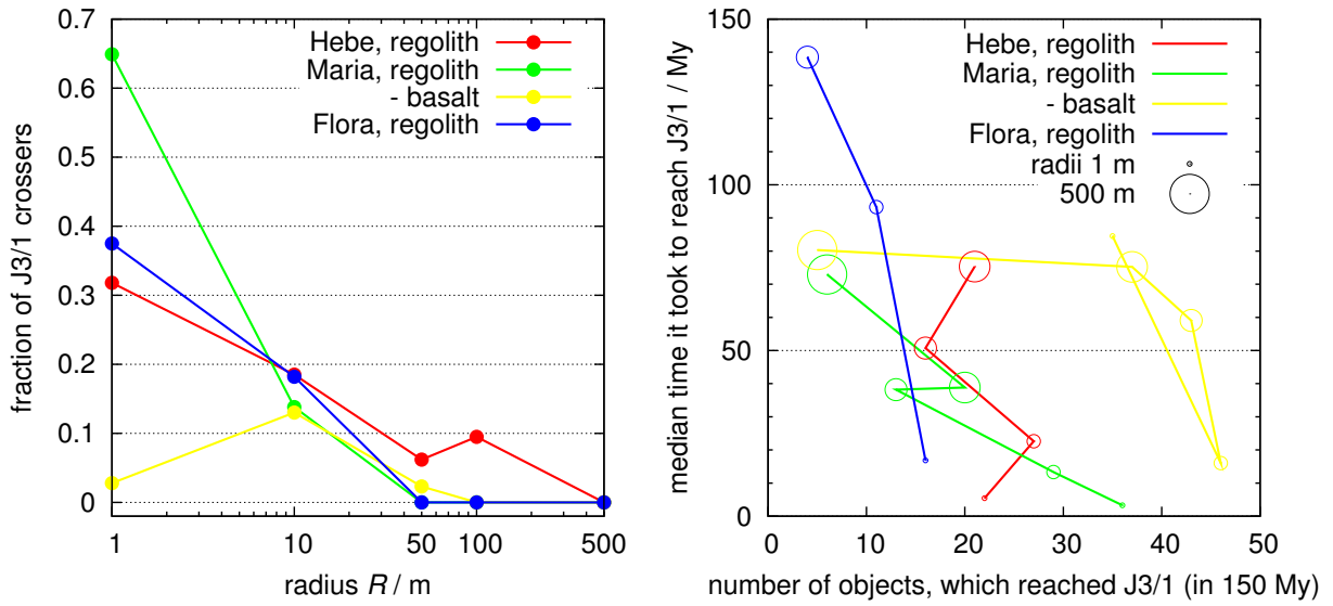
Figure 39: (Left) The fraction of the J3/1 crossers vs. their radius; the errors of the fraction are of the order 0.1 due to the limited number of meteoroids. (Right) The median time, it took to reach J3/1 resonance vs. the number of objects (out of 50), which actually did that within the time span of the integration (i.e., 150 My); the radii are indicated as sizes of the circles. The Hebe and Flora basalt meteoroids mostly drift away from the J3/1 resonance, hence we do not plot statistics for them.
