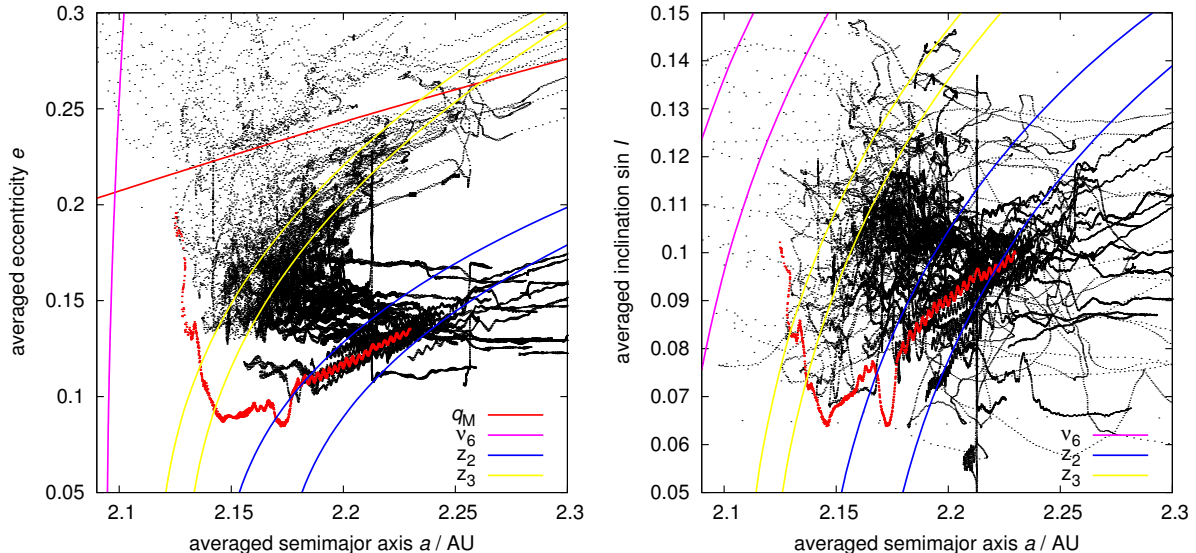
Figure 41: The role of high-order secular resonances in the orbital evolution of meteoroids: (left) the averaged semimajor axis vs. eccentricity for Flora 100 m regolith meteoroids, with captures in the z_2 resonance; (right) the semimajor vs. sine of inclination. The \pm 1 arcsec/y borders of the secular resonances were calculated using the secres8 program by A. Milani and Z. Knežević.
