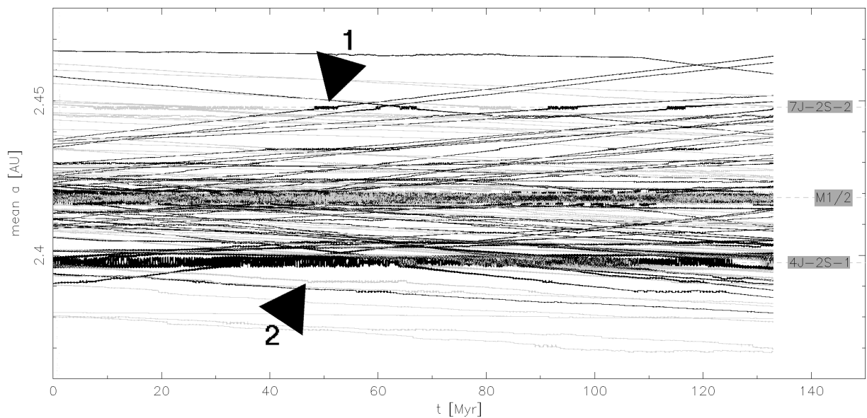
Figure 35: The orbital evolution of Hebe asteroid fragments with R = 500 m. Two types of bodies are plotted at once: regolith (dark) and basalt (light). We observe captures in the resonances M1/2, 4J-2S-1 and others. The arrow no. 1 points to the capture in the 7J-2S-2 resonance and the arrow no. 2 to an unidentified one (which decreases the drift rate slightly).
