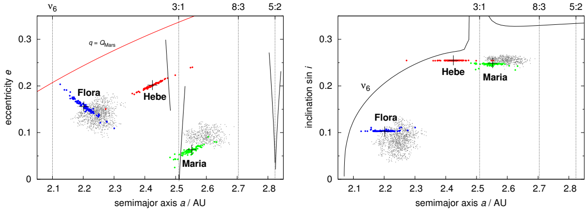
Figure 31: The parent bodies (crosses) and simulated ejecta (colour dots) at the osculating semimajor axis vs. osculating eccentricity plot. We draw also approximate positions of major gravitational resonances (black lines) and the Flora and Maria families (gray dots) in proper elements. We identified the Maria family by the hierarchical clustering method with a cutoff velocity v_{\text{cutoff}} = 70 m/s, using the AstDyS catalogue, version Nov 10 th 2004. The Flora family was identified at v_{\text{cutoff}} = 160 m/s among asteroids with H < 15 mag; for a larger dataset, it blends with the background population (for all velocities) and cannot be easily separated by the HCM algorithm.
