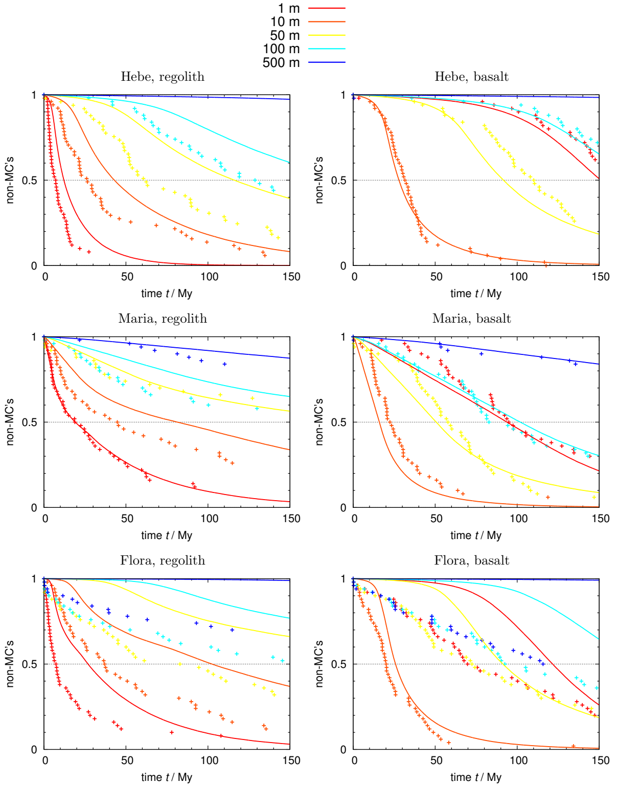
Figure 37: The ordinate gives a fraction of meteoroid population, which are not Mars crossers, vs. time for the three parent bodies and two materials. Colours denote radii: 1 m (red), 10 m (orange), 50 m (yellow), 100 m (cyan) and 500 m (blue). The crosses denote our N-body simulations (we use q < 1.665 AU Mars-crossing criterion, with 0.5 My averaging) and the lines correspond to simpler analytical Yarkovsky semimajor axis drifts and fixed resonant borders, which are used in the Monte-Carlo model by Vokrouhlický & Farinella (2000).
