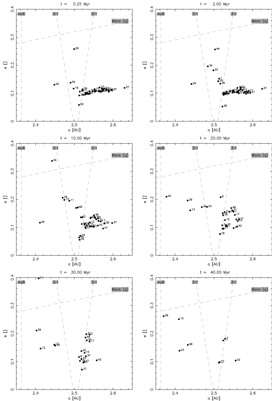
Figure 33: The evolution of 10 m basaltic meteoroids ejected from Maria displayed at the sequence of mean semimajor axis vs. mean eccentricity plots, spanning 40 My. Dashed lines denote approximate borders of the J3/1 resonance, the \nu_6 resonance and the Mars-crossing region. The group of meteoroids around no. 17 had been captured in the z_2 secular resonance before it entered J3/1 resonance.
