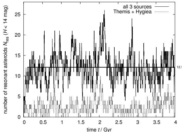
Figure 65: Estimated steady-state population of the unstable asteroids with H \leq 14 inside the J2/1 in our nominal simulation where all asteroids are assumed to have p_V = 0.05 . Fluctuations around the mean value of \simeq 12 are due to random injections into the resonance. The bottom dotted curve shows the contribution of the Themis and Hygiea families, \simeq 15\% of the total.
