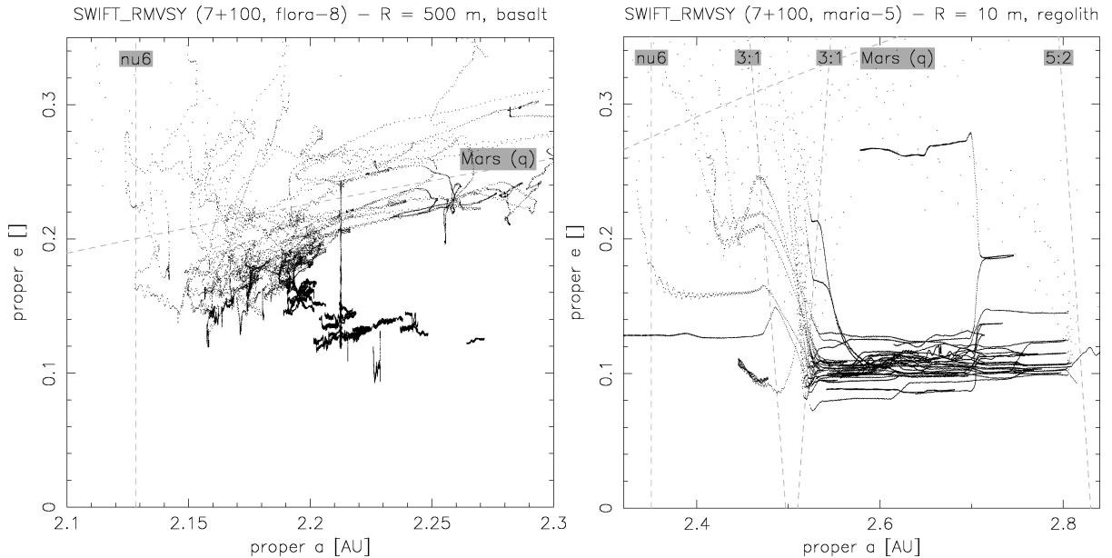
Figure 36: The averaged semimajor axis vs. eccentricity plots of the Flora 500 m basalt asteroid fragments (left) and Maria 10 m regolith meteoroids (right). There are many weak resonances in the inner belt, so slowly drifting bodies from Flora diffuse in eccentricity. The fast drifting bodies from Maria almost do not evolve in eccentricity unless they reach low-order resonances (J3/1, J5/2, J8/3 or \nu_6 ).
