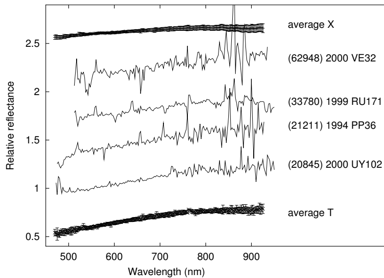
Figure 88: Relative reflectance spectra, normalized to unity at 550 nm, of asteroids in Table III. For (20845) UY102 the ordinate is in order, while for the other objects we arbitrarily shifted the data each time by 0.4 for visibility. For sake of comparison, we also show average reflectance spectra of T-type and X-type asteroids from the SMASS dataset (Bus and Binzel, 2002a,b, and http://smass.mit.edu/ ).
