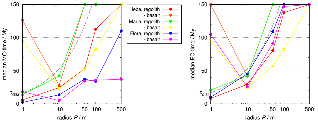
Figure 38: The dependence of the median Mars- and Earth-crossing times on the radius for regolith and basalt meteoroids originating from three parent bodies. Typical values are of the order 10 My, but the meteoroids drifting slowly or located far from the major escape routes have the median equal to 150 My (i.e., the time span of the integration), because less than half of the bodies ever reached MC (EC) orbits. The dashed curves indicate the characteristic disruption timescale \tau_{disr}(R) , given by Eq. (30).
