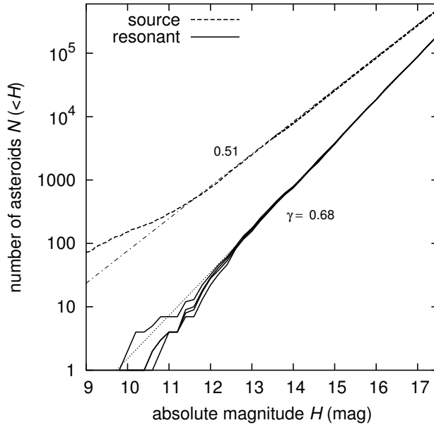
Figure 64: Cumulative H distribution of the simulated unstable population in the J2/1 (solid curves) compared with the source population (dashed curve). All 3 source populations are considered together. Large H values were found by extrapolating from small H values using a power law (compare the dashed curve with the dotted curve in Fig. 52). The 4 solid lines are distributions of resonant population collected during 2 Gy windows: 0.5 – 2.5 Gy, 1 – 3 Gy, 1.5 – 3.5 Gy and 2 – 4 Gy. They are nearly identical at small sizes but fluctuate at large sizes because some large asteroids occasionally fall in the resonance. Straight lines are local power-law approximations in the H range 12 – 14 (labels are the corresponding exponent value). Here we use our nominal model, A = A_{\text{nom}} and B = B_{\text{nom}} . All asteroids have the same albedo value p_V = 0.05 .
