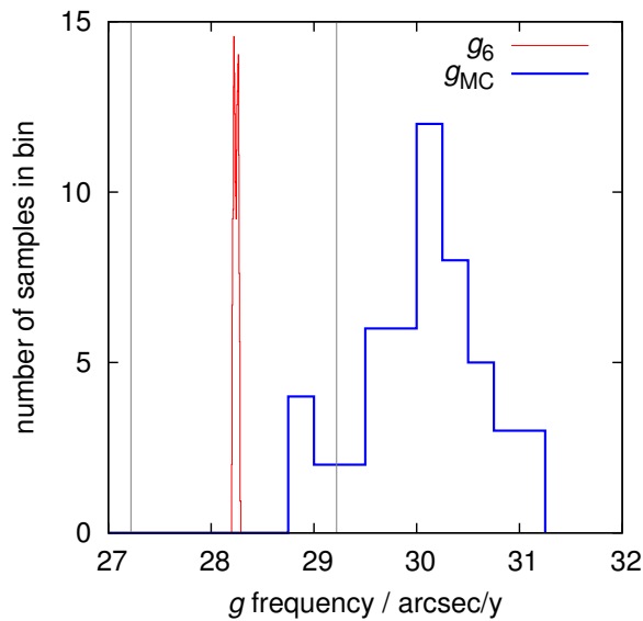
Figure 40: The histogram of the g_{MC} frequencies of meteoroids, i.e., the proper frequencies of longitudes of perihelia calculated by the FMFT method (see Section 9.1), at the moment when the meteoroids reach Mars-crossing orbits (according to the MC-criterion). The comparison to the g_6 frequency of Saturn is given, and the interval \pm 1 arcsec/y around the g_6 , i.e., the ‘area of influence’ of the \nu_6 resonance, is displayed as the two vertical gray lines. This calculation was performed for 50 Flora basalt meteoroids with R = 10 m.
