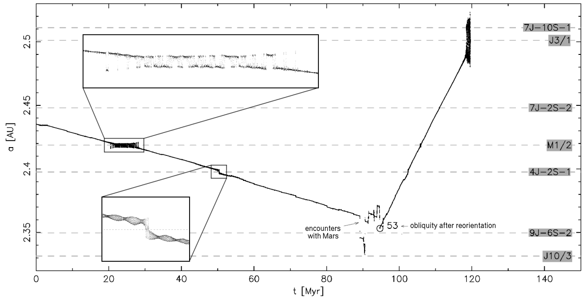
Figure 34: The orbital evolution of a Hebe 10 m regolith meteoroid at the mean semimajor axis vs. time plot. The capture in the M1/2 resonance and the jump over the 4J-2S-1 resonance are zoomed-in. The period of close encounters with Mars (around 90 Myr) was interrupted by a sudden reorientation of the spin axis, which caused a fast outward drift. Finally, the meteoroid reached the J3/1 resonance and was ejected from the Main Belt due to a close encounter with Jupiter.
