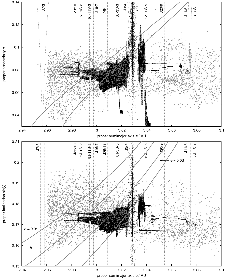
Figure 75: Evolution tracks of our synthetic Eos asteroids with size \geq 7 km during 1 Gy in our simulation; dots are \geq 7 km members of the currently observed family with the HCM threshold velocity V_c = 55 m/s. Top: proper eccentricity vs. proper semimajor axis; bottom: proper sine of inclination vs. proper semimajor axis. The initially compact family extends in course of time due to a combination of the (i) Yarkovsky forces that produce diffusion in the semimajor axis, and (ii) interaction with MMRs that, upon capture, cause eccentricity and inclination to change. The latter effect is proportional to the resonance strength scaling with its order. Thus the principal resonances –here J9/4– make many of the captured asteroids eliminated from the family. Weaker MMRs, such as 16/7 or the three body resonances (shown in the figure), do not have a capability to eliminate asteroids from the family, yet they can make the family to extend in eccentricity and inclination. A special effect is produced by the high-order secular z_1 resonance (Sec. 6.3.3) that make the Yarkovsky drifting orbits frequently captured and driven along it for a long period of time. This is because this resonance varies along all proper elements, approximately diagonally across the family. The grey curves show nominal location of the resonance \pm 0.8 “/y zone for: (i) \sin i = 0.17 (top), and (ii) e = 0.04 and e = 0.08 (bottom). The particle moving toward small proper eccentricity value at \sim 3.02 AU shows a rare temporarily capture in a weak secular resonance g - 3g_6 + 2g_7 .
