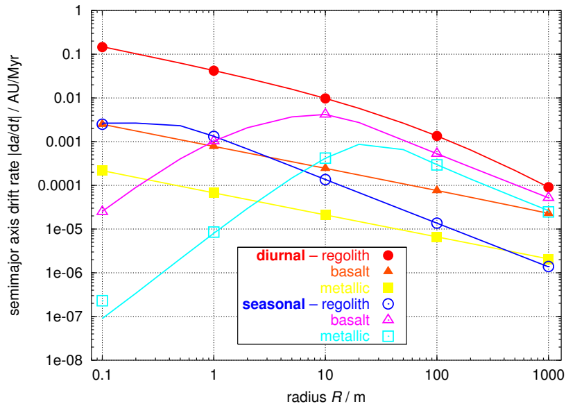
Figure 107: The absolute values of the semimajor axis drift rates da/dt (in AU/Myr) for particles with several values of radii (from 0.1 m to 1 km) and three different types of thermal parameters: regolith, basalt and metallic-like. The initial orbits of test particles were a = 2 AU, e = 0 , i = 0^\circ . The two variants of the Yarkovsky acceleration (diurnal and seasonal) are plotted separately. The lines correspond to the analytic estimates, the points are computed numerically by a LSM fit of the output a(t) .
