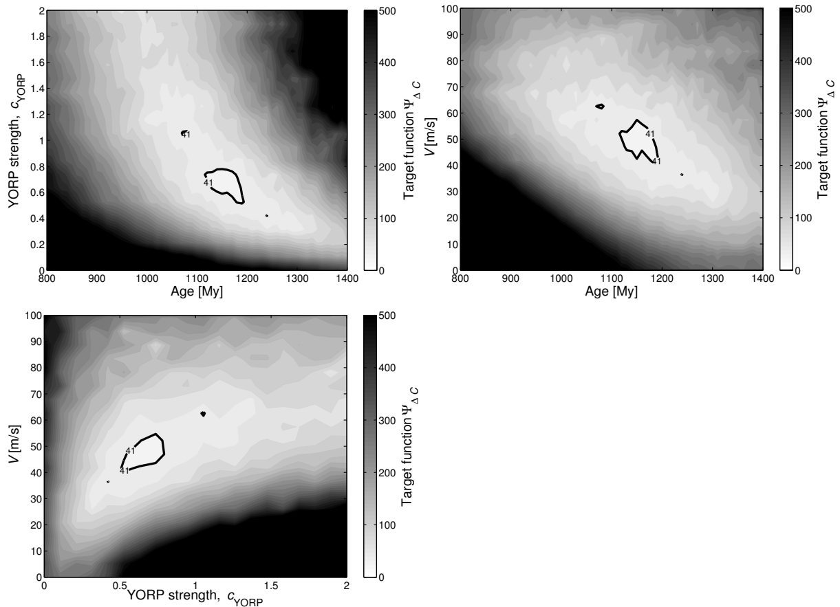
Figure 82: Projection of the target function \Psi_{\Delta C} onto planes defined by the model parameters: (a) T vs. c_{\text{YORP}} , (b) T vs. V , and (c) c_{\text{YORP}} vs. V (as in the previous figure V_{\text{SD}} = V is size-independent). Each time we plot the smallest \Psi_{\Delta C} value along the ray of the third parameter (i.e. in the first case we fix T and c_{\text{YORP}} values of seek the minimum value for all tested values of V ). We show shaded contours of \Psi_{\Delta C} with the value indicated by a bar on the right; the best fit value is \Psi_{\Delta C} = 27.8 . This compares to 41 bins in \Delta C , which set the formal 1\sigma uncertainty level (shown in bold curve).
