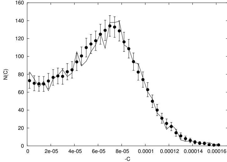
Figure 80: Comparison of the observed and modeled distribution \mathcal{D}(C) for the Eos family; here we use model with size-independent velocity V_{\text{SD}} that characterizes dispersal of the initial fragments along all directions. We actually show directly number N_{\text{obs}}(C) , and N(C) , of asteroids within a strip (C, C + \Delta C) for \Delta C = 4 \times 10^{-6} AU used in the target function \Psi_{\Delta C} in Eq. (50). Symbols are the observed bodies N_{\text{obs}}(C) with the assigned formal uncertainty \sqrt{N_{\text{obs}}(C)} ; only the left branch of the family with asteroids having a \leq a_c is used here. This is an averaged result where a_c is assumed to be uniformly distributed in the range (3.015, 3.025) AU. Broken solid line is our modeled family that minimizes the target function \Psi_{\Delta C} .
