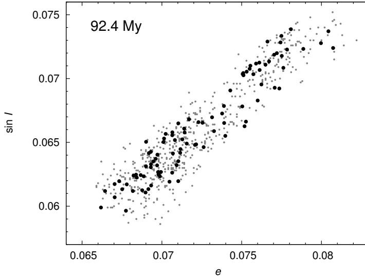
Figure 102: The nominal Agnia family members projected onto the plane of proper eccentricity e and inclination \sin i (light symbols) and the configuration of of numerically integrated sample of bodies at time 92.4 My when the Kolmogorov-Smirnov probability of their coincidence shows a maximum. Both distributions indicate concentration toward extreme values of the proper elements and depletion near their mean values for the family. This effect occurs periodically due to libration cycle in the z_1 resonance.
