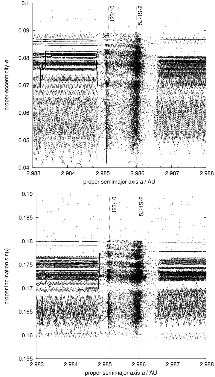
Figure 77: A zoom of the Fig. 75 showing tracks of particles in our simulation near a pair of weak mean motion resonances J23/10 and 5J-1S-2 (see the text for nomenclature); dots are the currently observed asteroids. Upper panel is a projection onto the proper eccentricity vs. proper semimajor axis values, lower panel gives a projection onto the proper sine of inclination vs. proper semimajor axis values. Because of the Yarkovsky forces the orbits migrate toward smaller semimajor axis values. Upon encounter the mean motion resonances, the proper eccentricity might be significantly changed; the inclination effect is quite less for these resonances. The bottommost migrating particles are trapped in the z_1 secular resonance and stay so even after a period of interaction with the mean motion resonances.
