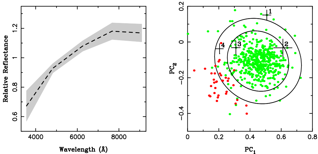
Figure 91: Left: Dashed curve shows a mean 5-color spectrum for 499 small Eos members from the SDSS database (release 3.0; see Jurić et al., 2002 and http://www.astro.princeton.edu/~ivezic/sdssmoc/sdssmoc.html ) whose principal spectral components have an error smaller than 0.1 (here we normalized the result to unity at 550 nm as conventional). The shaded zone shows a standard deviation interval about the mean. Right: The Eos family members (light symbols) projected onto the plane of spectral principal components PC_1 and PC_2 (e.g. Nesvorný et al., 2005a); here we use again the sample of 499 asteroids observed with SDSS with small enough errors. The two ellipses show a 90% (inner ellipse), resp. 99% (outer ellipse), confidence level of a formal relation between the two components that define the Eos family as a cluster of data in these variables. Objects outside these limits are likely alien to the family. Here we list large members in this zone: (i) 1 – (8340) Mumma, (ii) 2 – (1755) Lorbach, (iii) 3 – (4843) Megantic, and (iv) 4 – (4431) Holeungholee; the horizontal and vertical intervals show error-bars of the data. The last two were classified X-types by the narrow-band spectroscopy, while (8340) Mumma received D classification and (1755) Lorbach T classification (see Fig. 89). For sake of comparison we also show the neighboring Veritas family (dark symbols), classified as C-type group.
