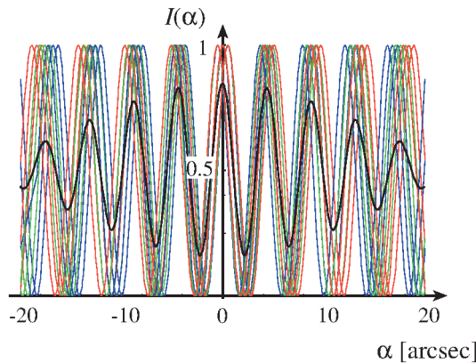
d) extended source, K-band
