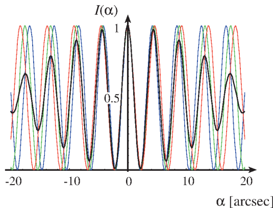
b) point source, K-band
