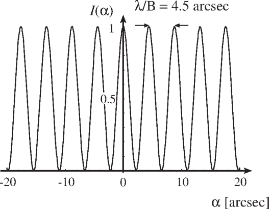
a) point source, monochromatic
