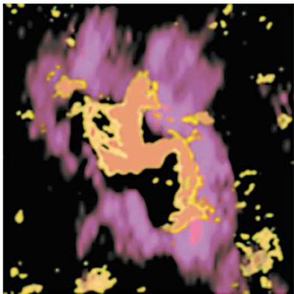
Wright et al. 1993 Yusef-Zadeh, Melia & Wandle 2000
