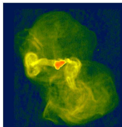
M87 – VLA (90 cm), \sim 70 kpc
