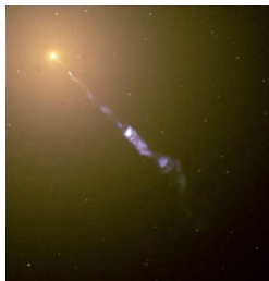
M87 – HST, \sim 2 kpc
