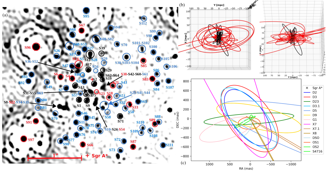
Figure 1.2 Observational overview of the S-cluster and compact objects orbiting Sgr A*. Left: Adaptive-optics infrared image of the central arcsecond, showing the projected positions of S-stars relative to Sgr A* (taken from Ali et al. (2020)). Individual stars are labeled, and the location of Sgr A* is marked. Top right: Three-dimensional orbital solutions for selected S-stars, illustrating the high eccentricities and orientations of their orbits (taken from Ali et al. (2020)). Bottom right: Projected orbital fits for a sample of dust-enshrouded sources, highlighting their close periaapse passages and diverse orbital properties (taken from Peißker et al. (2024b)). This population of young stars and dusty objects within \sim 40 mpc of Sgr A* presents strong constraints on formation and dynamical evolution scenarios in the Galactic Centre.
