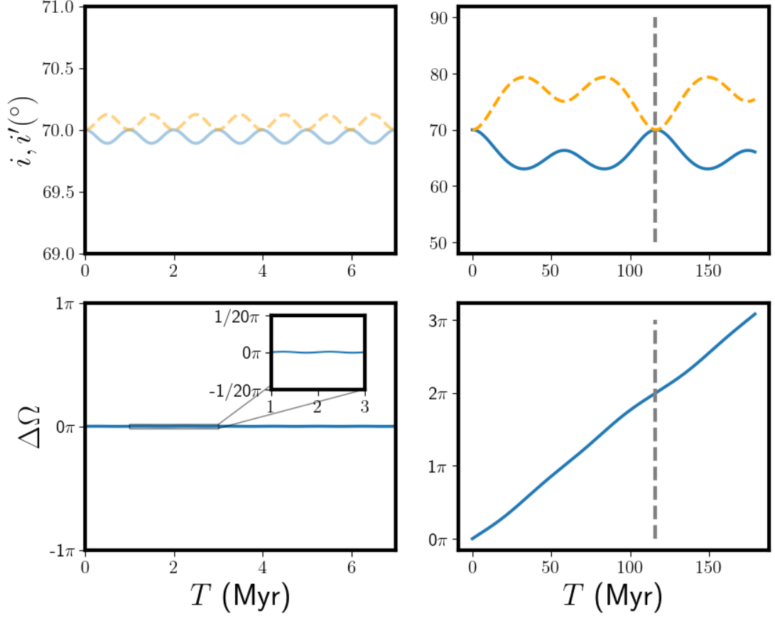
Figure 2.2 Orbital evolution of two mutually interacting light bodies orbiting a central massive object under the influence of a distant perturber, as described by the VHS mechanism. The left panels illustrates the synchronized precession of the longitude of ascending nodes ( \Omega ) in the ‘strong mode,’ with small scale oscillations in mutual inclination which preserves the initial co-planar structure of the bodies. The right panels demonstrates the ‘weak mode,’ where independent precession leads to large-scale oscillations in mutual inclination.
