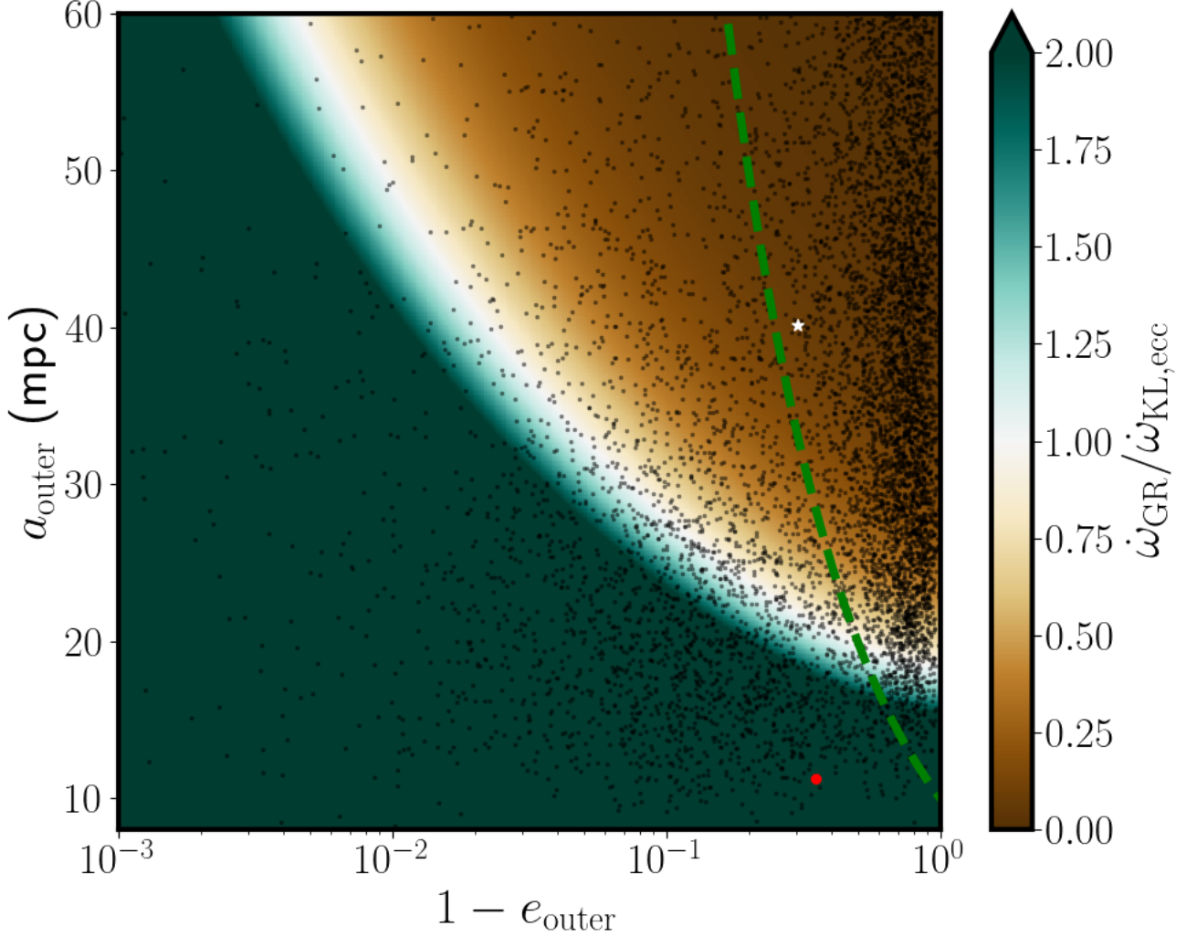
Figure 6. In the heatmap we show the ratio of \dot{\omega}_{\text{GR}}/\dot{\omega}_{\text{KL}} for the outer orbit of the binary system around SgrA* at a_{\text{outer}} with an eccentricity of e_{\text{outer}} . The perturber is a single particle mimicing the center of mass of the disk M_{\text{pert}} = 24500 M_{\odot} orbiting at a_{\text{pert}} = 0.12 \text{ pc} with an eccentricity of e_{\text{pert}} = 0.44 . The region where \dot{\omega}_{\text{GR}}/\dot{\omega}_{\text{KL}} \gtrsim 1 is where we expect KL oscillations to be completely damped while for the rest of the parameter space we expect KL oscillations to be undamped. Black dots mark the orbital parameters of merging binaries with M_c \leq 20 M_{\odot} . Red dot marks the orbital parameter of a star that undergoes KL oscillations with GR in a numerical simulation as showed in Figure 7. The green dashed line represents where r_{\text{p, outer}} = 10 \text{ mpc} . The white star marks the starting location of the binary shown in Figure 10.
