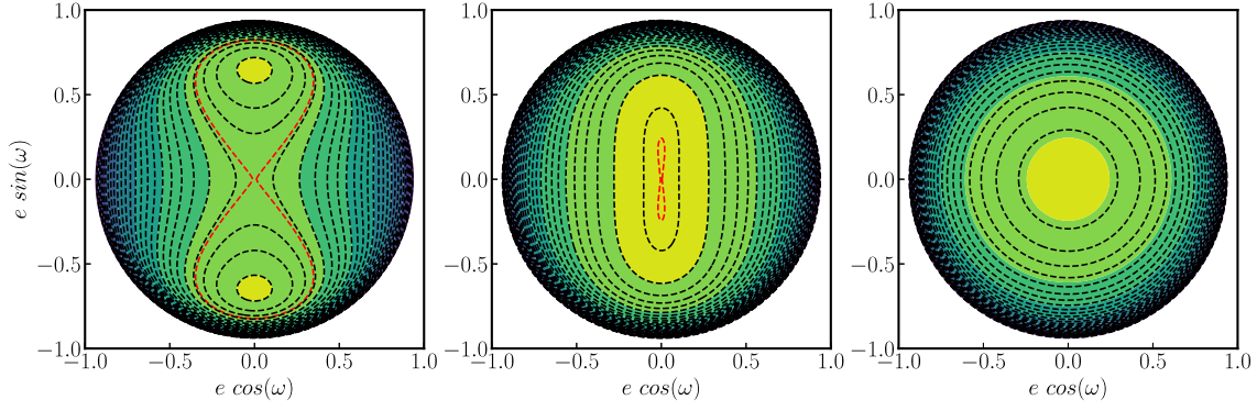
Figure 2. The potential isolines when the potential due to post-Newtonian approximation is added to the perturbing potential are displayed in three panels, representing two cases with identical parameters except for the semimajor axis of the test particle. In these examples, the value of C = 0.34 which is smaller than the limiting value for K-L dynamics, and the separatrix is shown in red. The panel on the left depicts the instability at e = 0 when a = 0.2R_p , while the panel on the right illustrates the stability at e = 0 when a = 0.03R_p . The central panel shows the boundary area when a = 0.145R_p and the K-L oscillations are damped.
