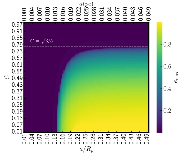
Figure 3. Heat map of largest variation in eccentricity for a 1 M_\odot star initially on an orbit of eccentricity e = 10^{-4} in the combined potential of a central dominant body ( M_\bullet = 4 \times 10^6 M_\odot ) and a distant perturber ( M_p = 10^4 M_\odot and R_p = 0.1 \text{ pc} ) on a circular orbit. The lower value of maximum eccentricity in a significant range of the parameter space shows that the relativistic corrections due to the SMBH partially or entirely dampen the K-L oscillations.
