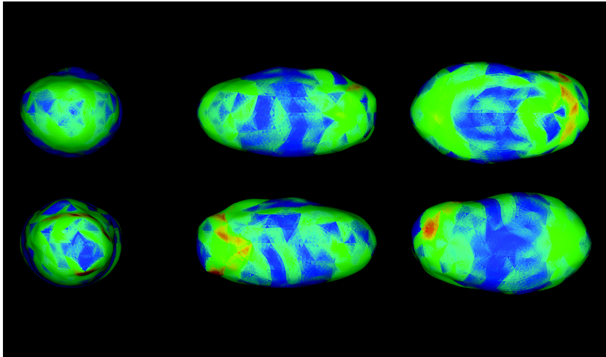
Radar model of asteroid 25143 Itokawa, color-coded for gravitational slope.
