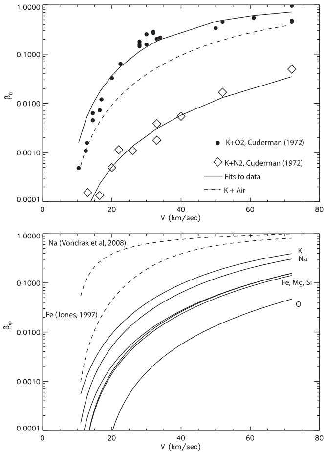
Figure 19. Top: \beta measured by Cuderman (1972) for K + O 2 and K + N 2 . The solid lines through the experimental points are fits of the expression from Jones (1997). The dash line is the estimated \beta_0 for K + air collisions, which includes the correction for multiple high energy collisions. Bottom: variation of \beta_{ip} for all the meteoric atoms colliding with air, as a function of particle velocity.
