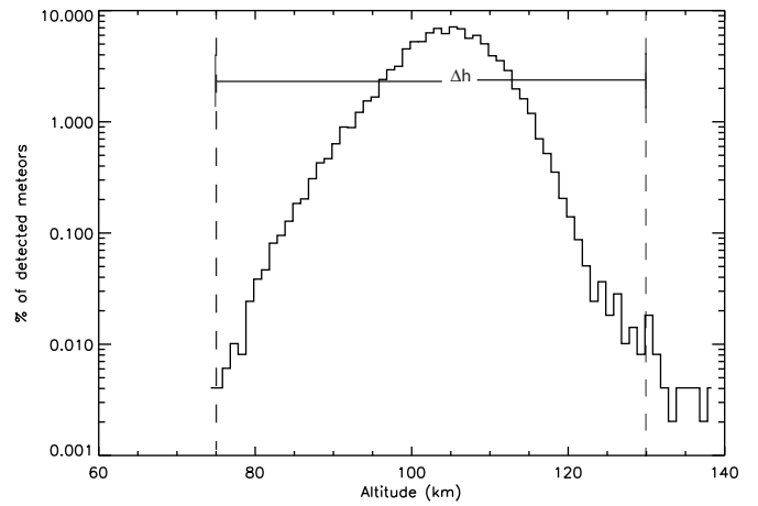
Figure 12. Observed altitude distribution with the Arecibo radar during the 2002 observing campaign. Observations are clearly present in the 75–130 km altitude range, which results in \Delta h = 55 \text{ km} .
