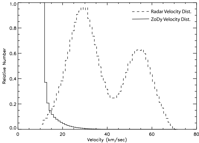
Figure 1. Solid line shows the velocity distribution resulting from ZoDy (Nesvorný et al. 2010). The dashed line represents the velocity distribution at the top of the atmosphere generally measured by radars (Fentzke & Janches 2008).
